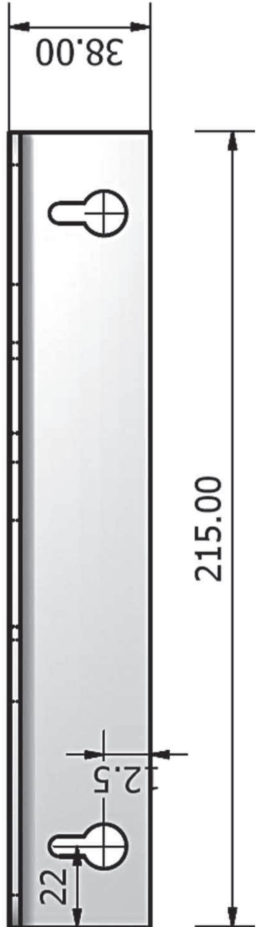
Figure 1. Template to place holes for screws.
